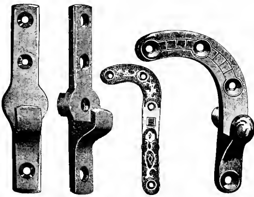
Figs. 4051-4052. STRAIGHT SEAT-ARM STOPS.
